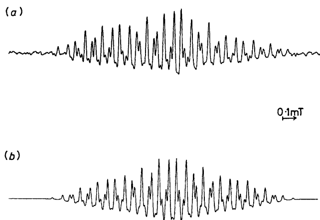
Figure 2. (a) 9.4 GHz second-derivative e.s.r. spectrum of dimeric radical (21) obtained from the ^{13}\text{C} -labelled pyrrolone (15); (b) simulation, using parameters given in the Table
