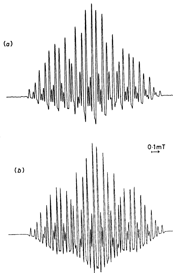
Figure 1. (a) 9.4 GHz second-derivative e.s.r. spectrum of dimeric radical (21) obtained from the pyrrolone (12); (b) simulation, using parameters given in the Table
